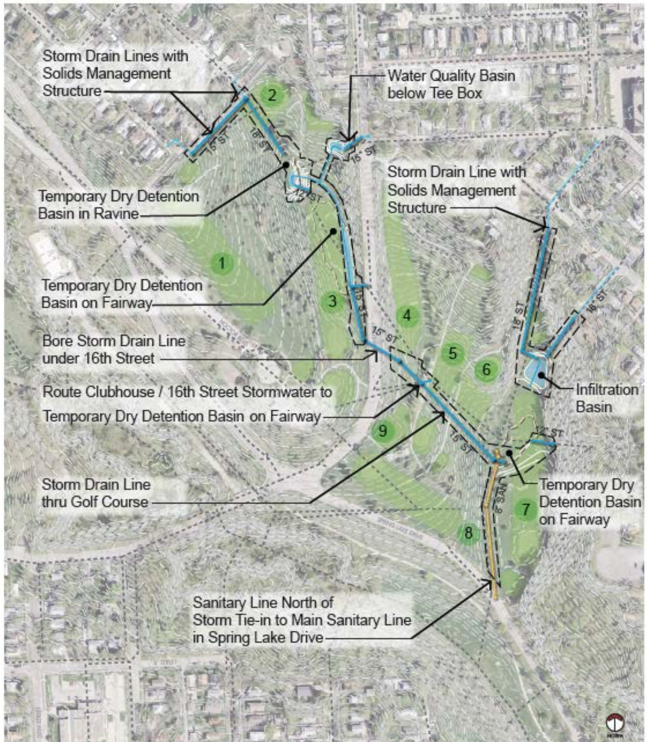
Missouri Avenue Sewer Separation alignments – September 2016 Spring Lake Park Neighborhood Meeting
